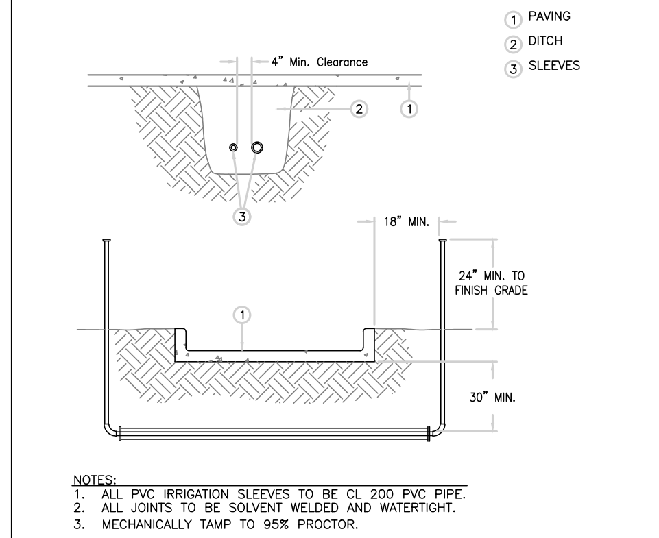
O SLEEVING
