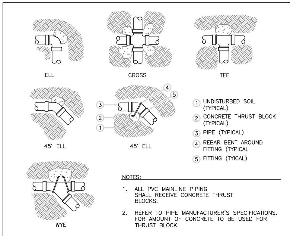
L THRUST BLOCK
