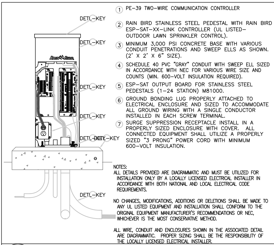
C RAIN BIRD SAT CONTROLLER
