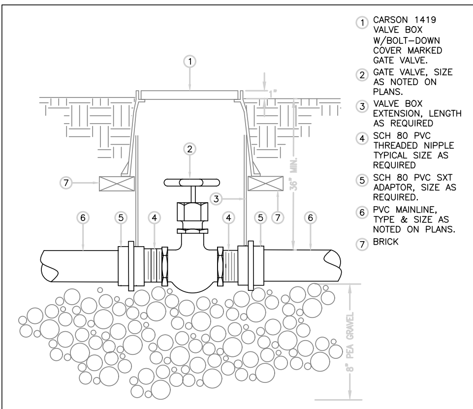
D T-113 GATE VALVE
