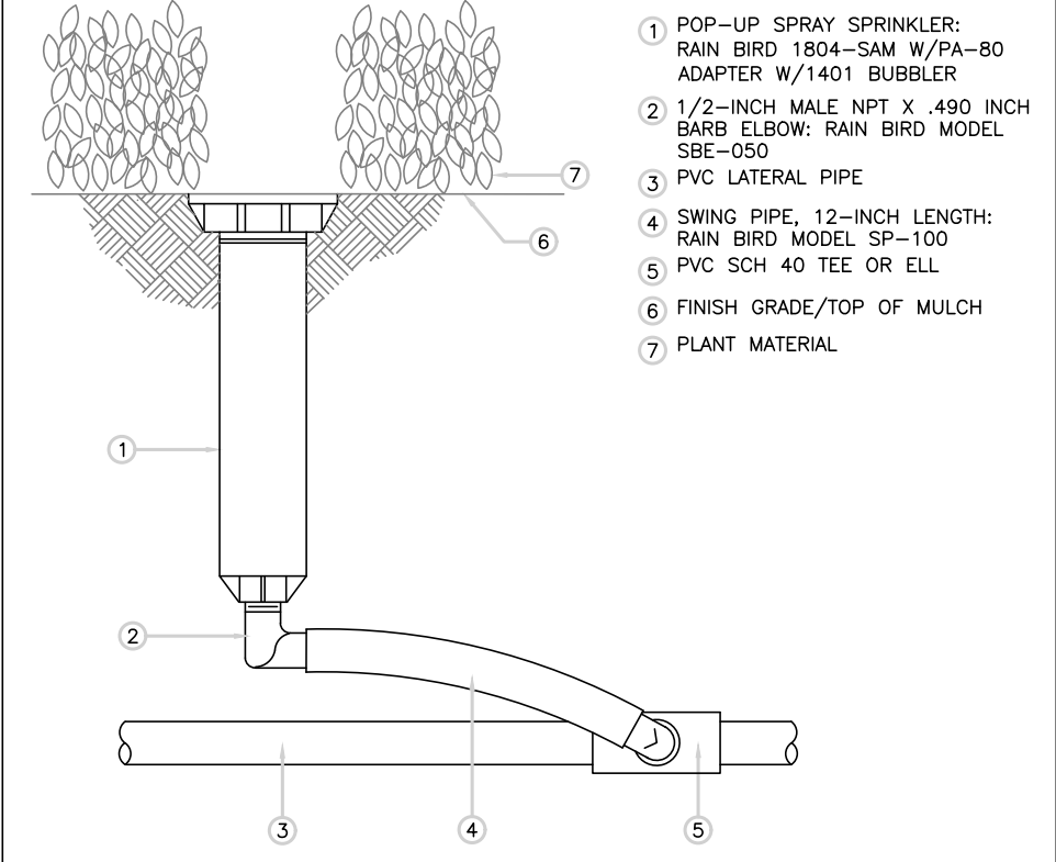
Q RAIN BIRD 1804-SAM POP-UP WITH 1401 BUBBLER
