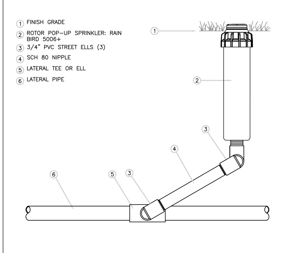
V RAIN BIRD 5000 GEARED ROTOR
