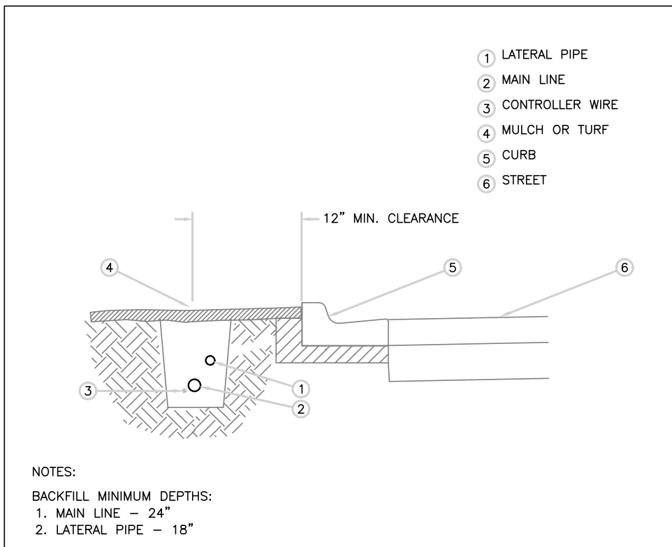
L MAINLINE AND LATERAL PIPING DETAIL
