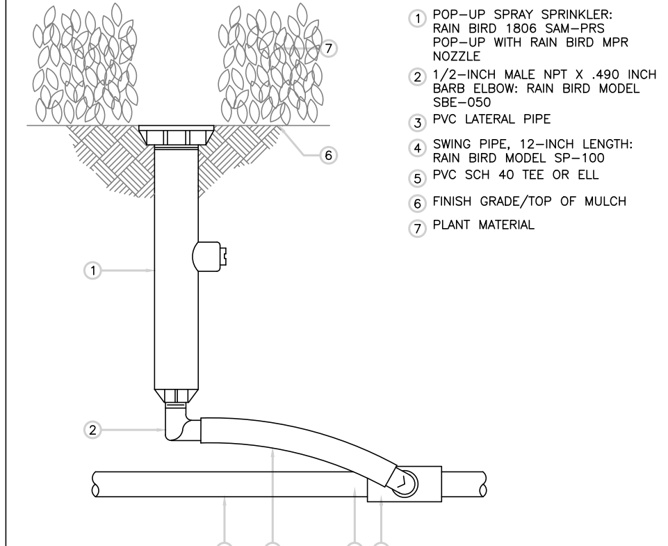
R RAIN BIRD 1806 SAM-PRS SPRAY
