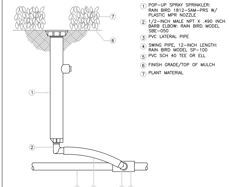
S RAIN BIRD 1812 SAM-PRS SPRAY
